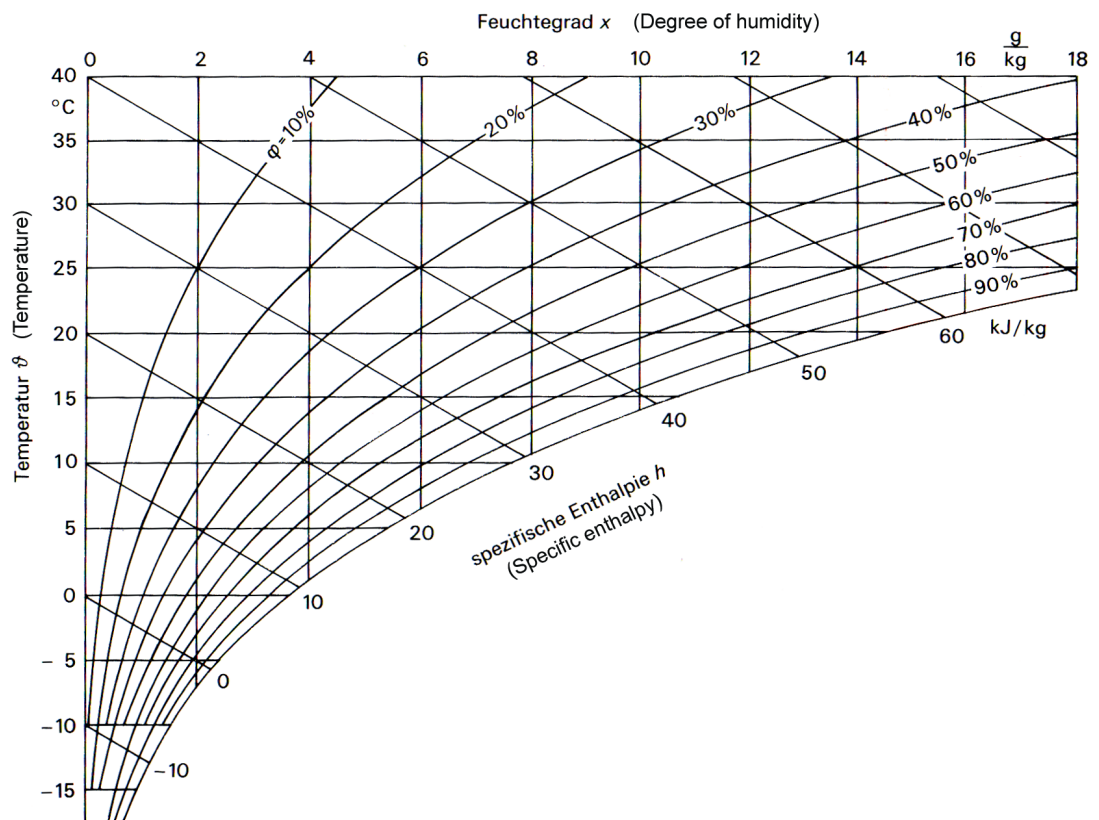
Mollier h/x diagram
